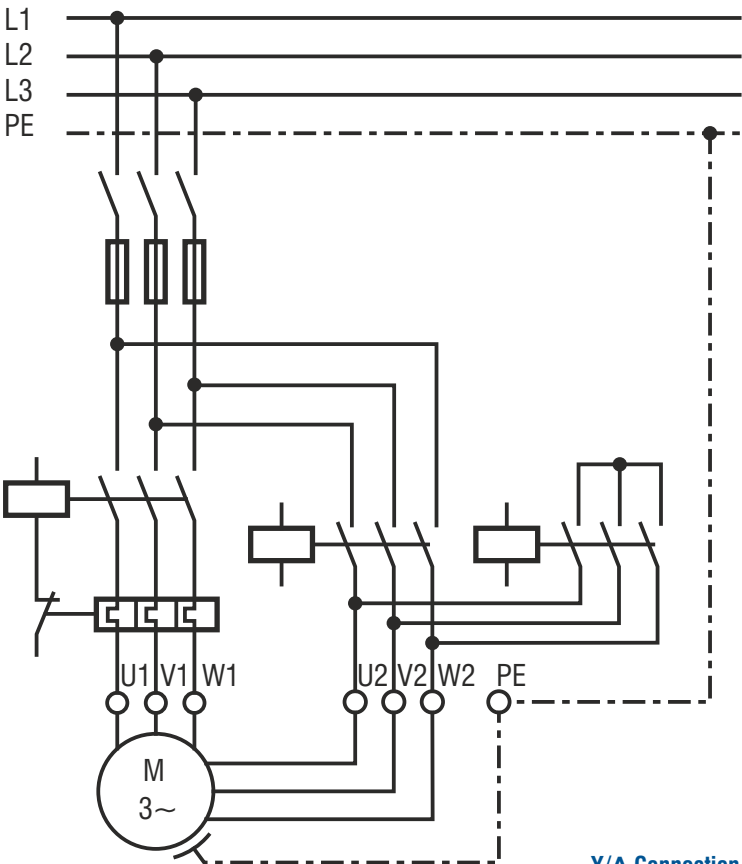
Y/Δ Connection
